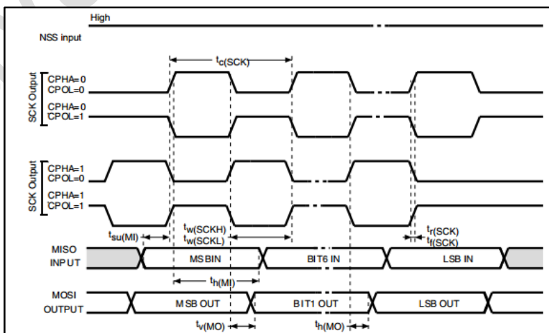
Figure 5-8 SPI Timing Diagram-Master Mode(1)
